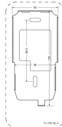
Drilling Template
